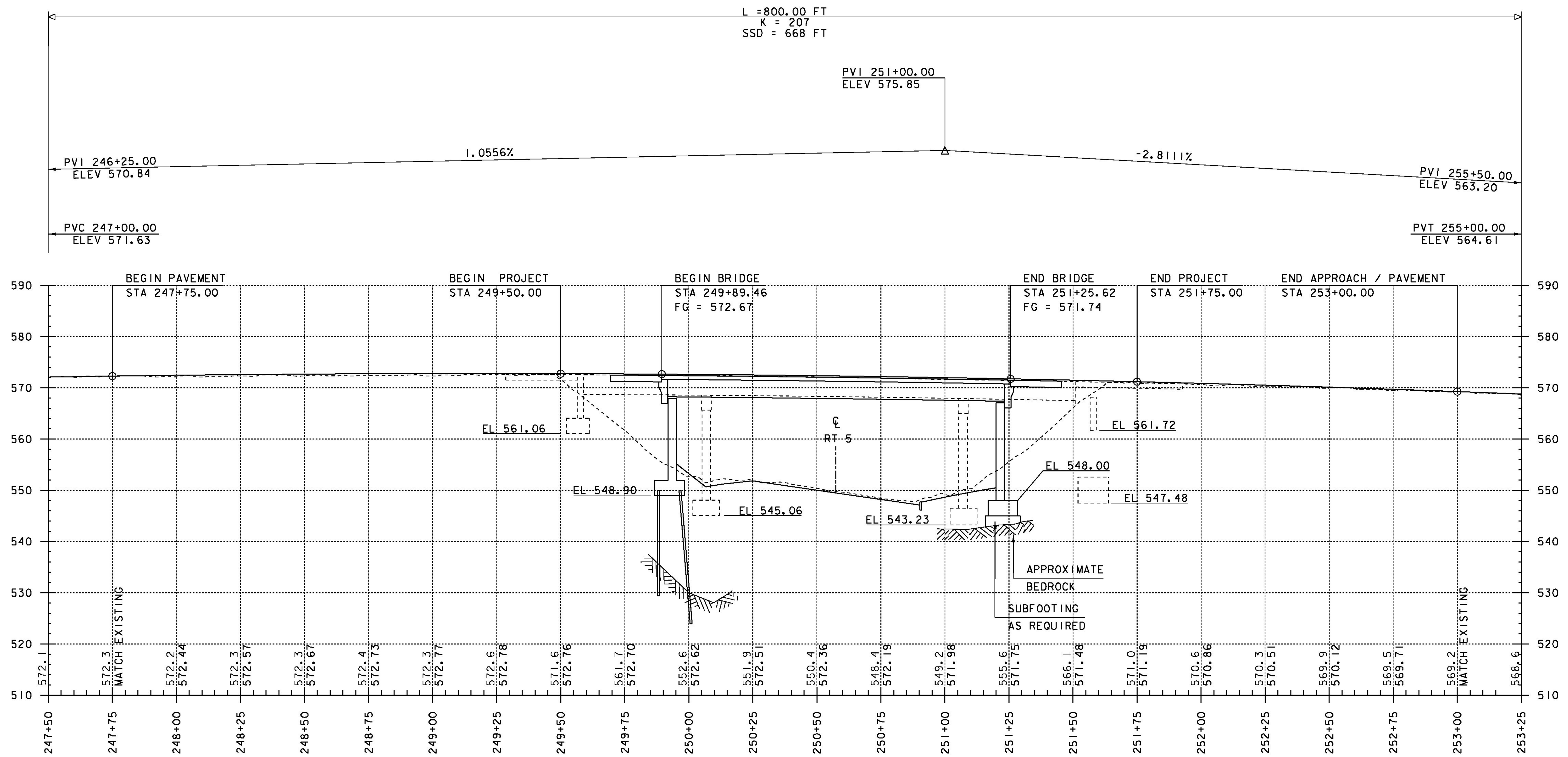
I-91 NB PROFILE HOR. SCALE 1" = 20'-0" VER. SCALE 1" = 10'-0"
