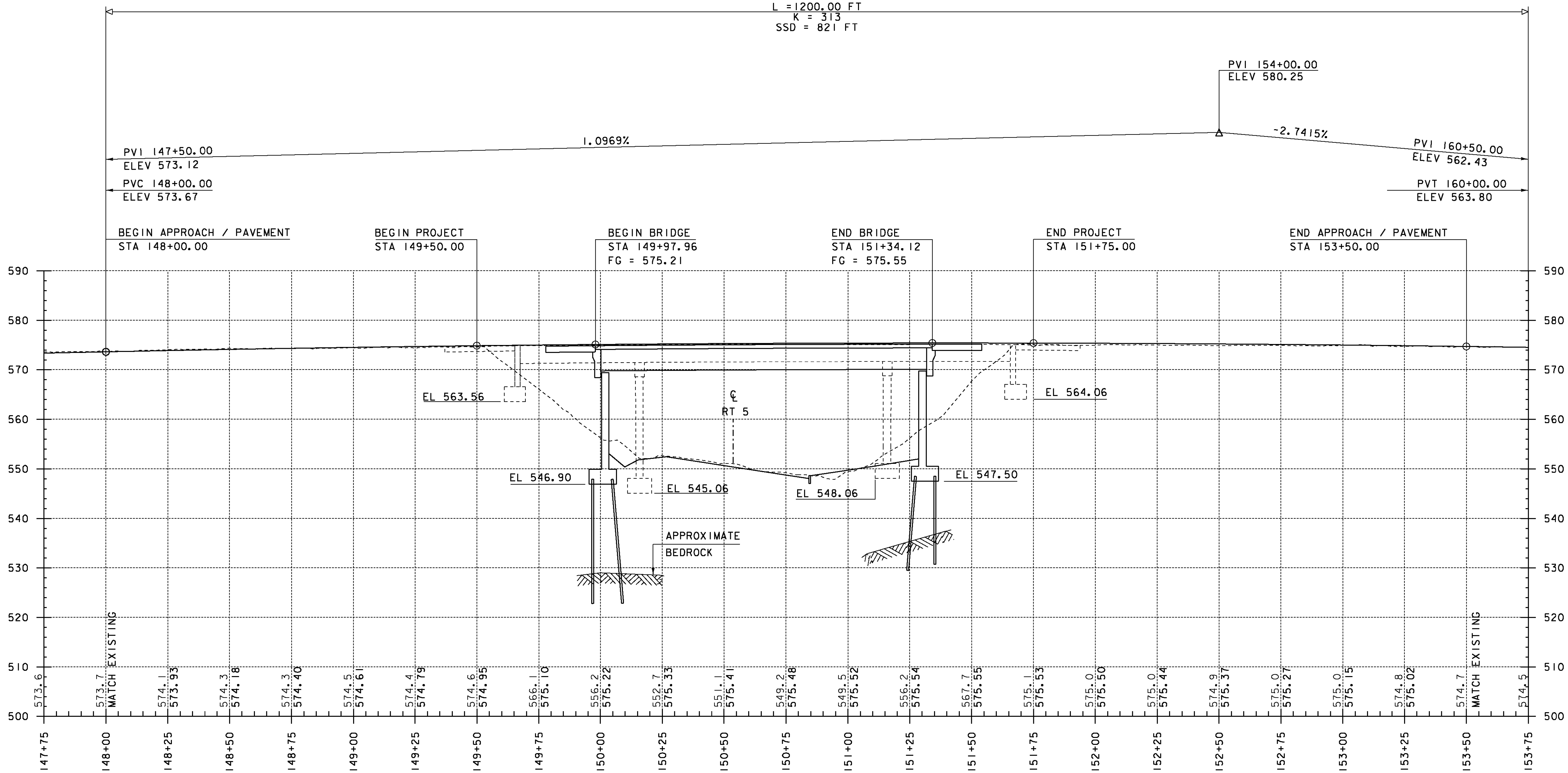
I-91 SB PROFILE HOR. SCALE 1" = 20'-0" VER. SCALE 1" = 10'-0"
