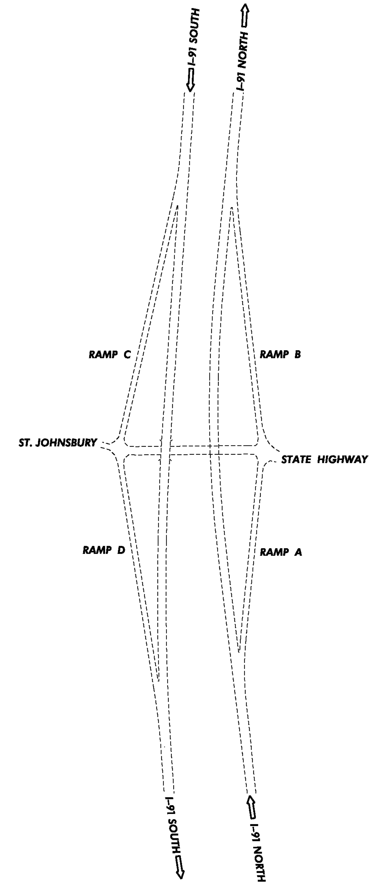
EXIT 22 LAYOUT
