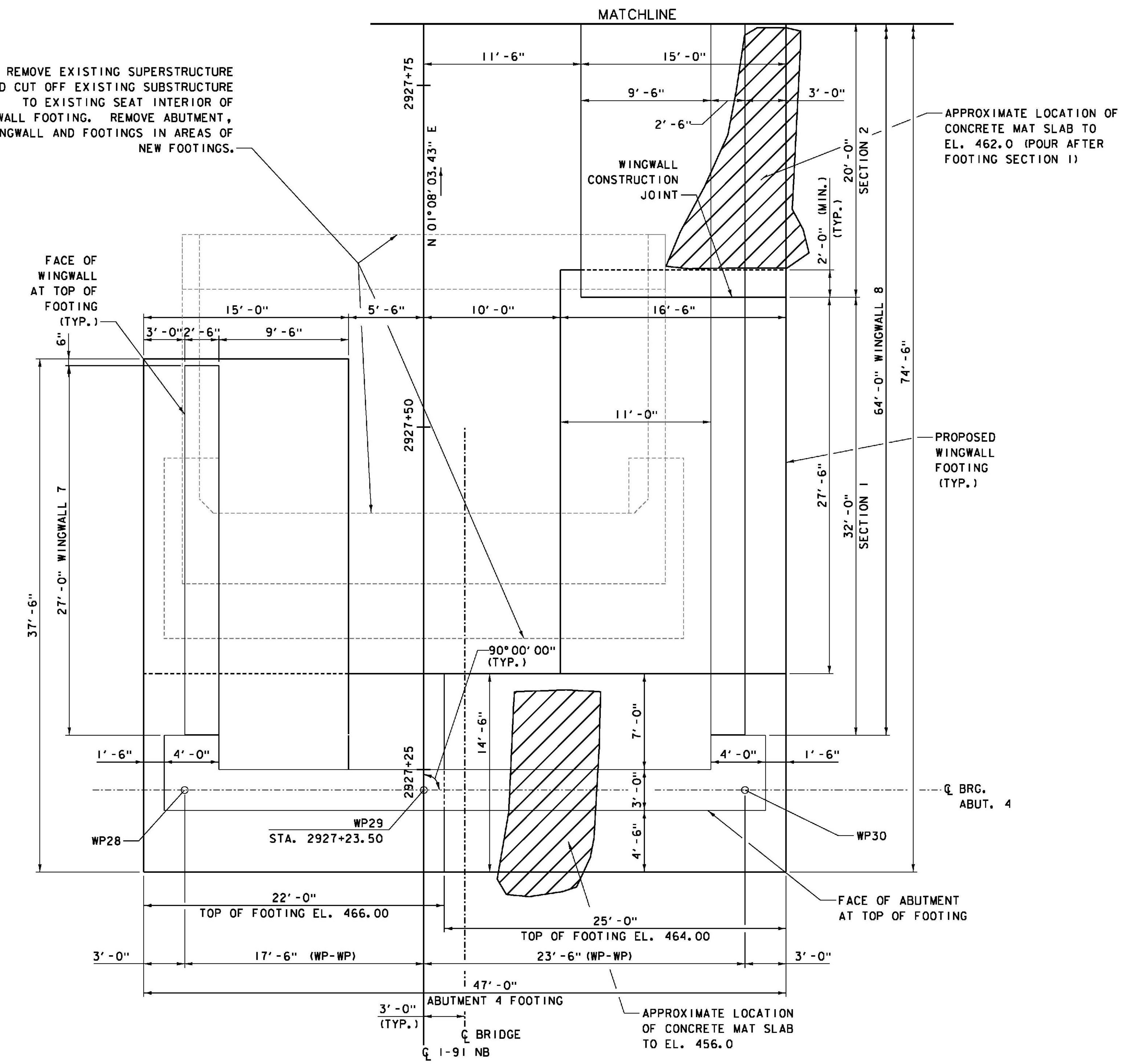
ABUTMENT 4 FOOTING PLAN SCALE 1/4" = 1'-0" 0 2 4 6
