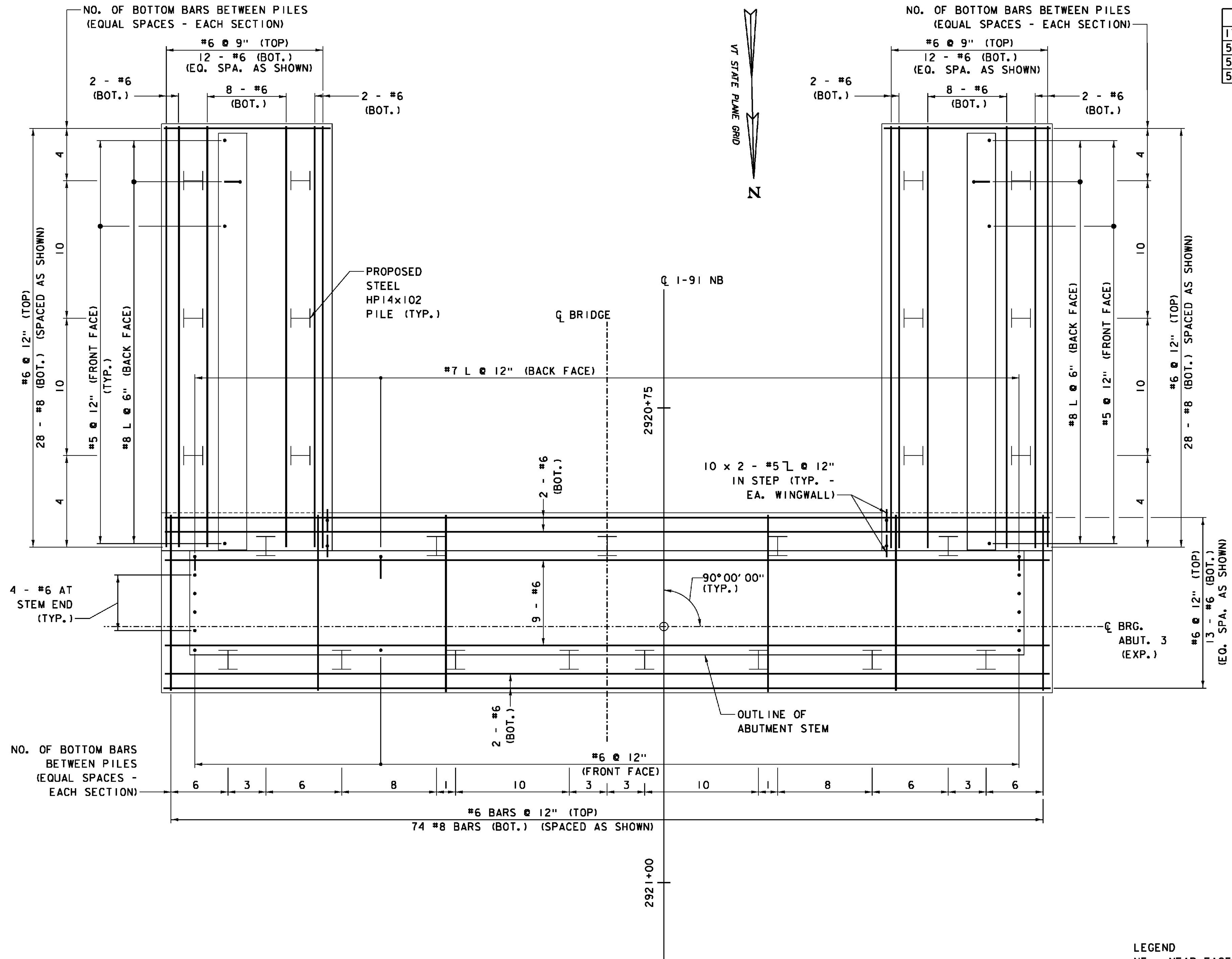
ABUTMENT 3 FOOTING REINFORCEMENT SCALE 3/8" = 1'-0" 1 0 1 2 3 4
