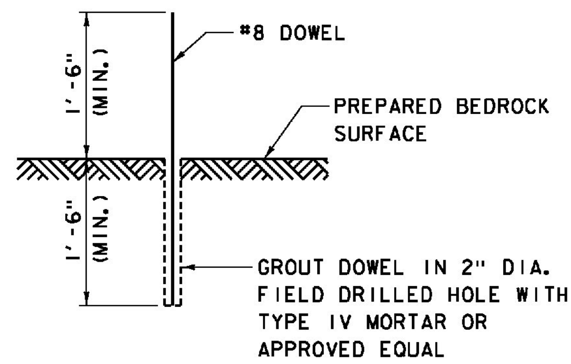
TYPICAL FOOTING DOWEL DETAIL NOT TO SCALE
