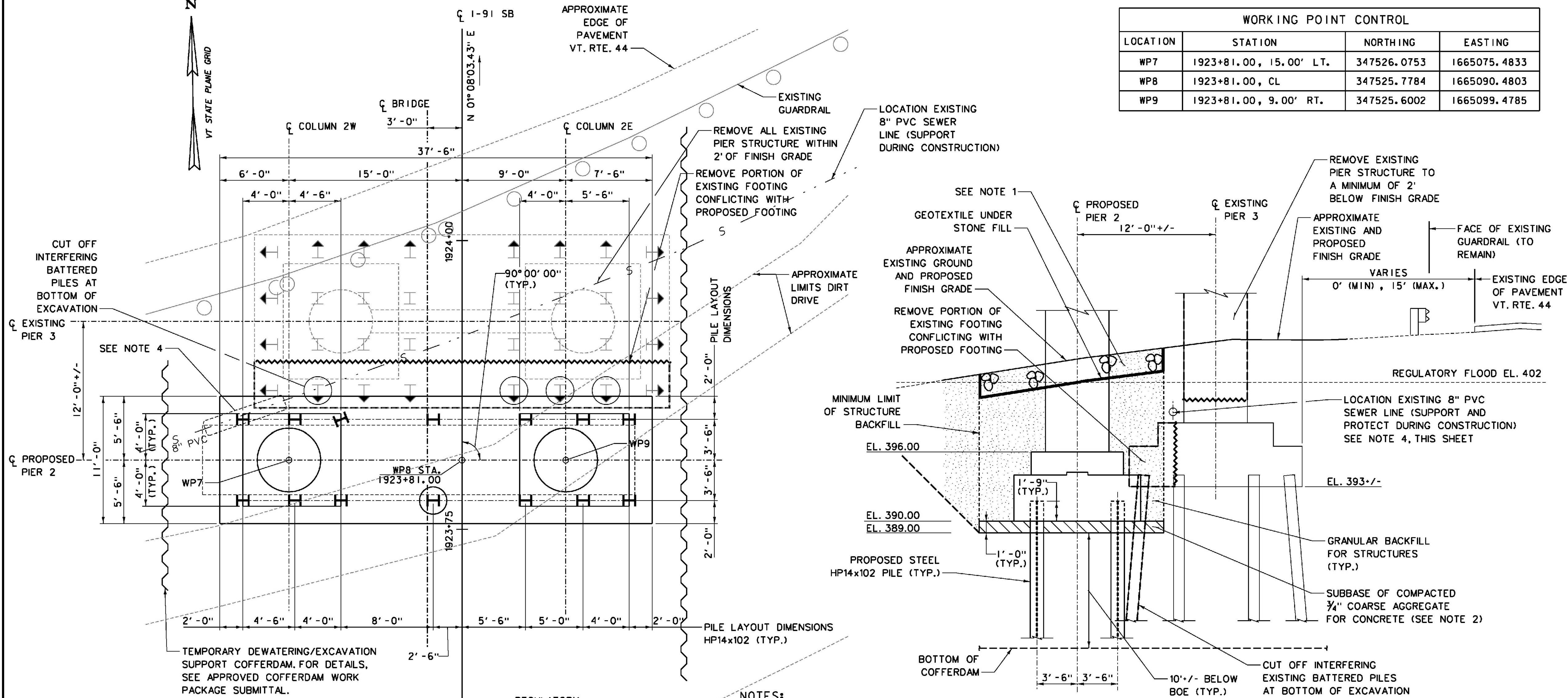
PIER 2 FOOTING SECTION SCALE 1/4" = 1'-0"
