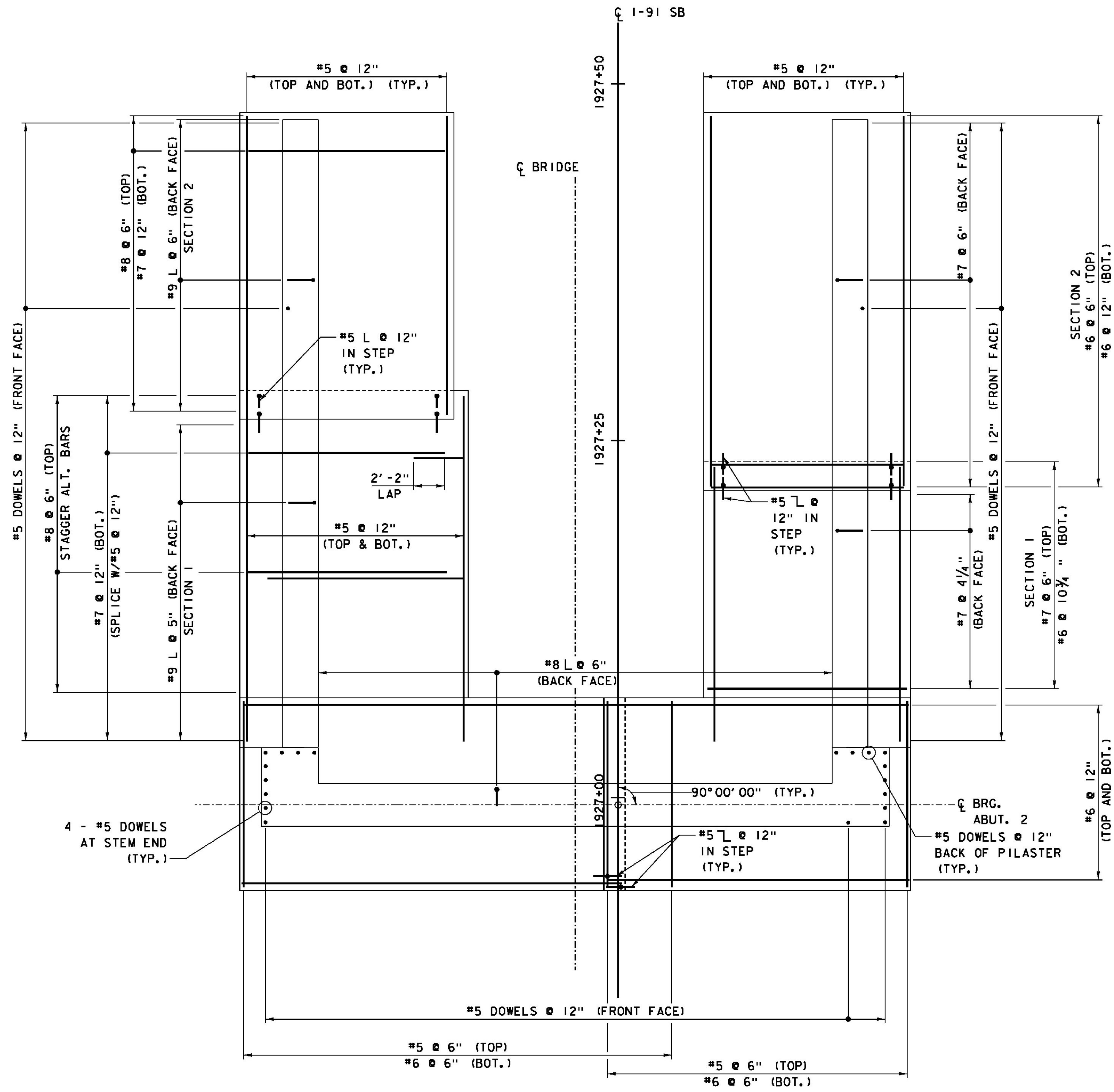
ABUTMENT 2 FOOTING REINFORCEMENT
