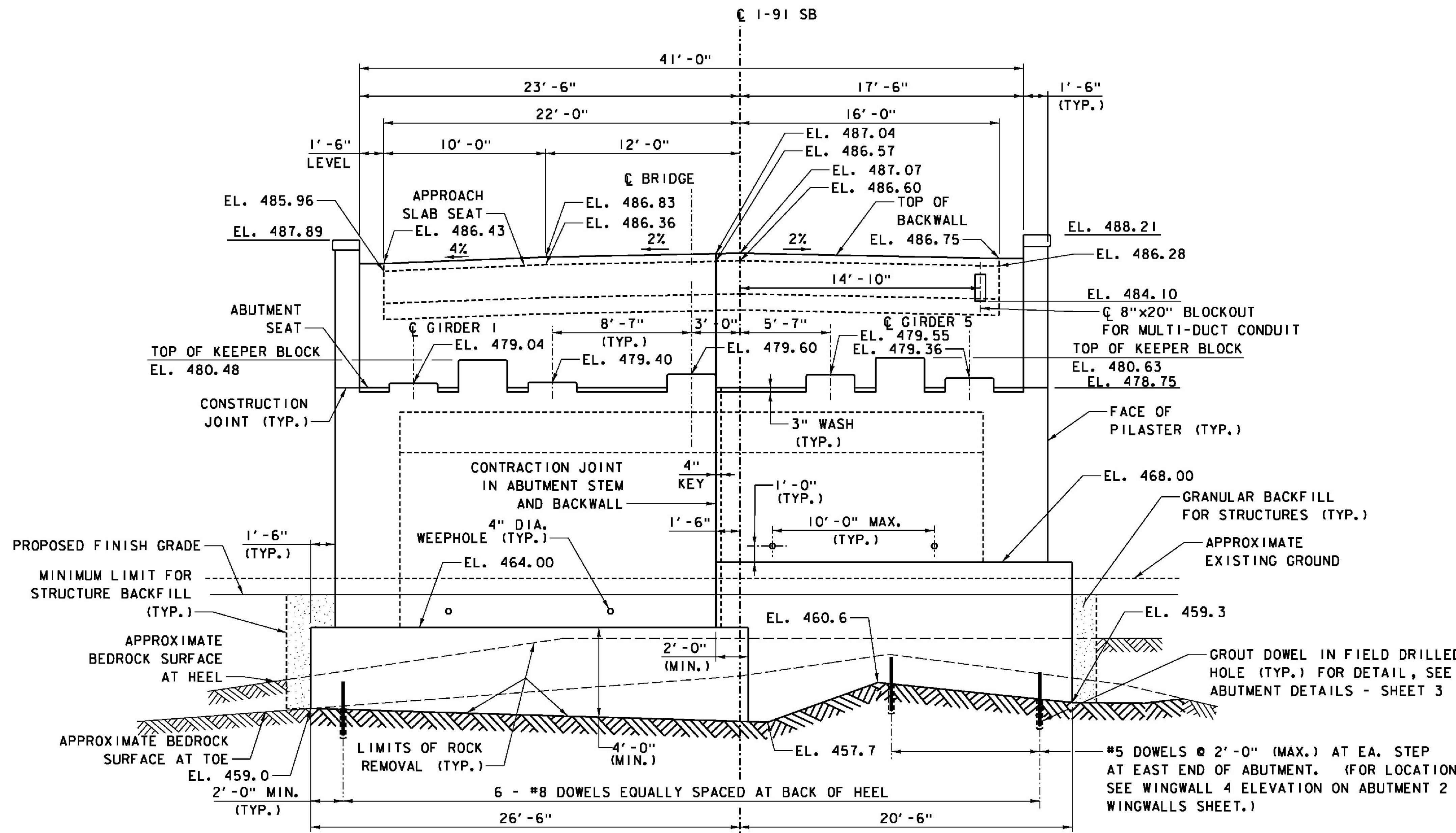
ABUTMENT 2 ELEVATION SCALE 1/4" = 1'-0" 1 0 2 4 6
