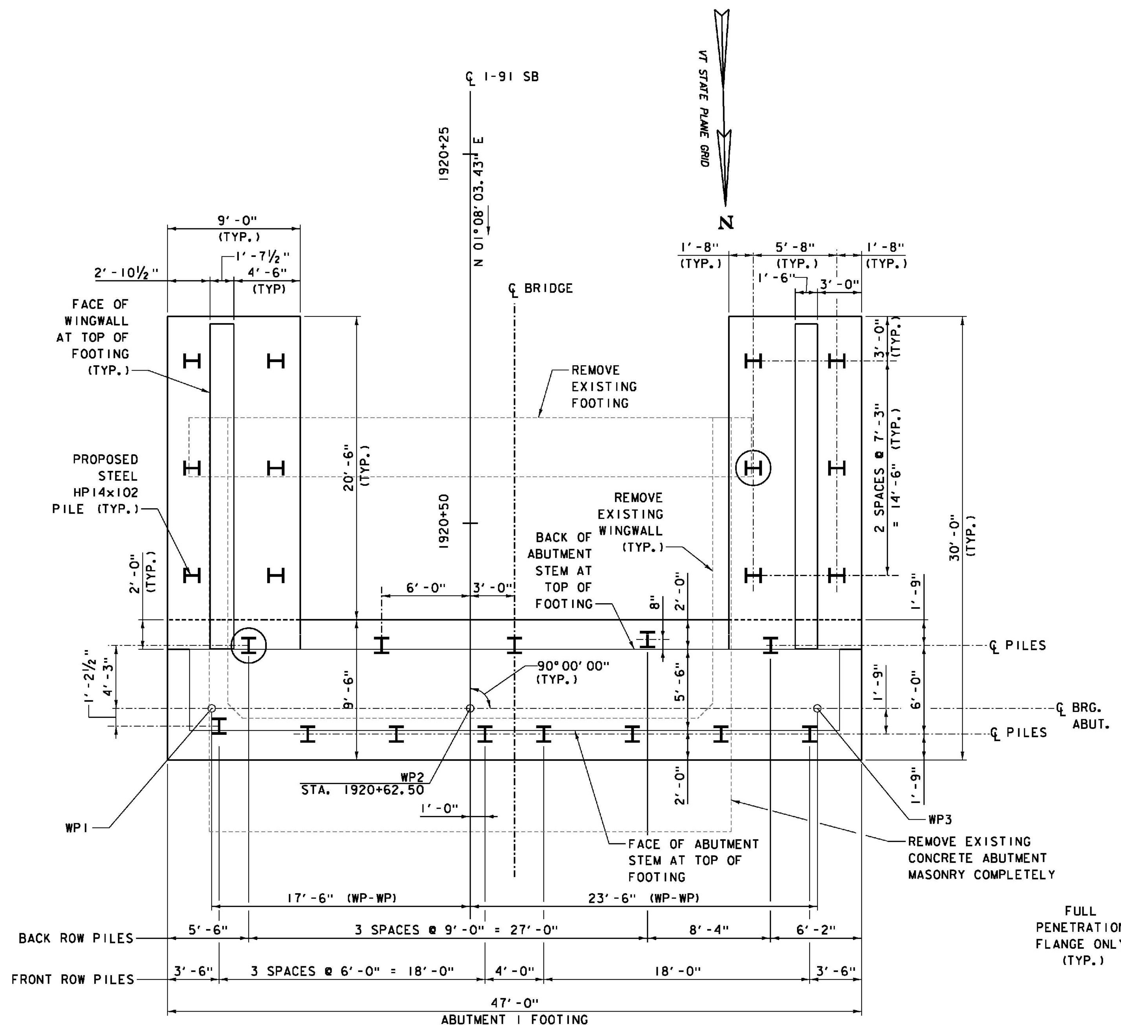
ABUTMENT 1 FOOTING PLAN
