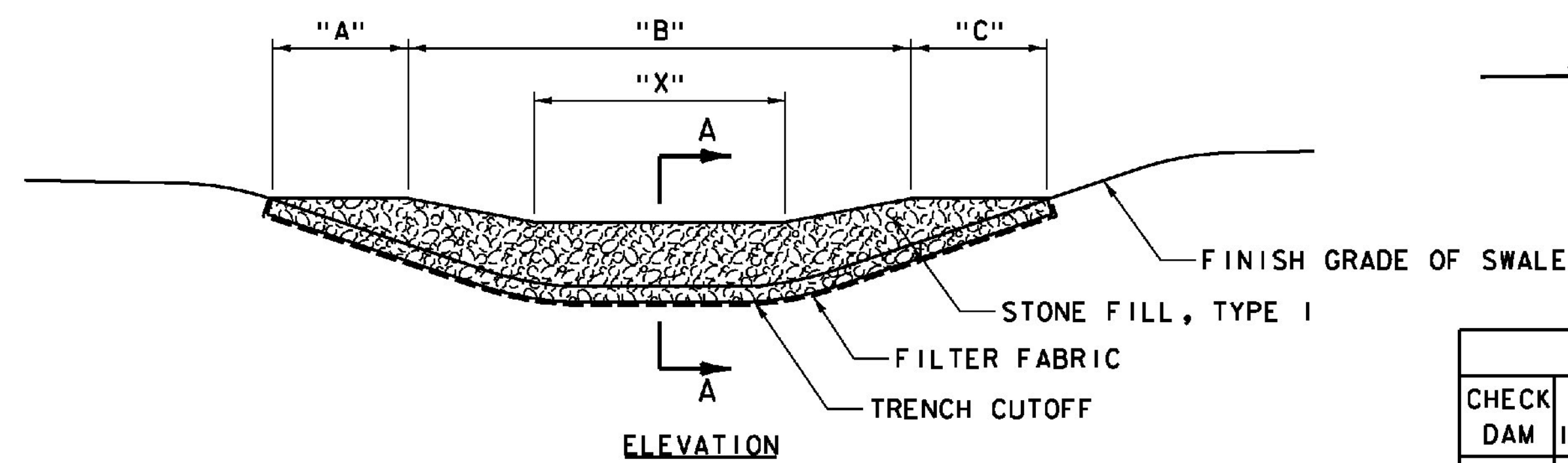
CHECK DAM WITHIN DRY SWALE SCALE 1/4" = 1'-0"
