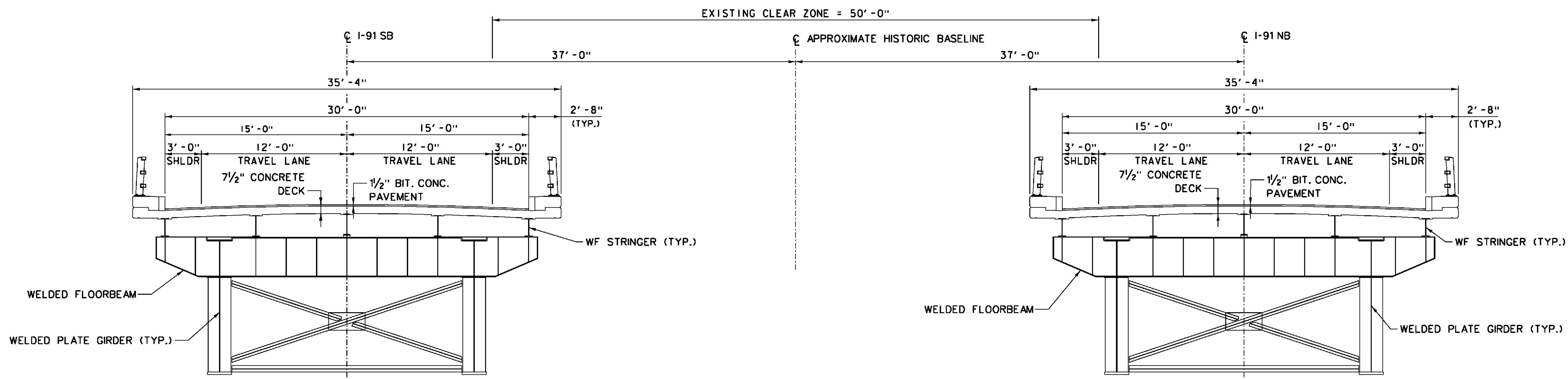
EXISTING TRANSVERSE SECTION
