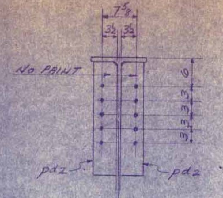
SECTION B-B TYPICAL DIAPHRAGM CONNECTION AT PIERS
