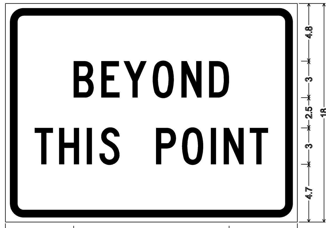
1.5" Radius, 0.6" Border, 0.4" Indent, Red on White; *BEYOND" C; *THIS POINT" C;
