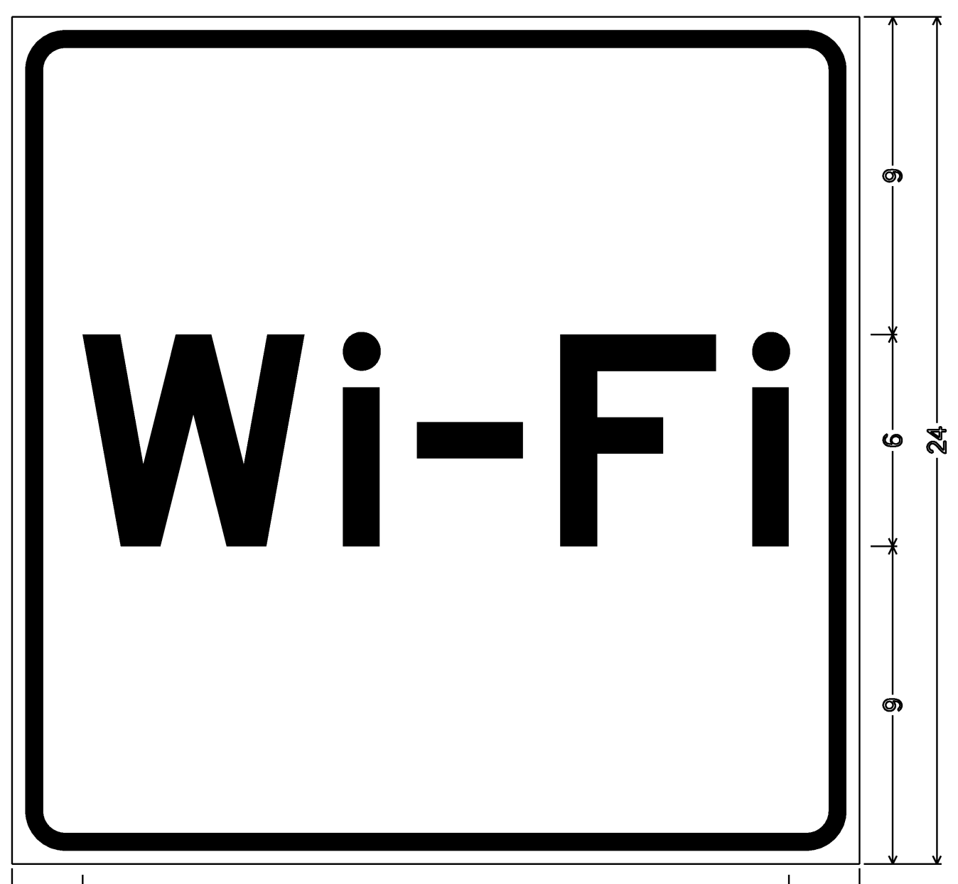
1.50" Radius, 0.50" Border, 0.38" Indent, White on Blue; *Wi-Fi" E specified length;
