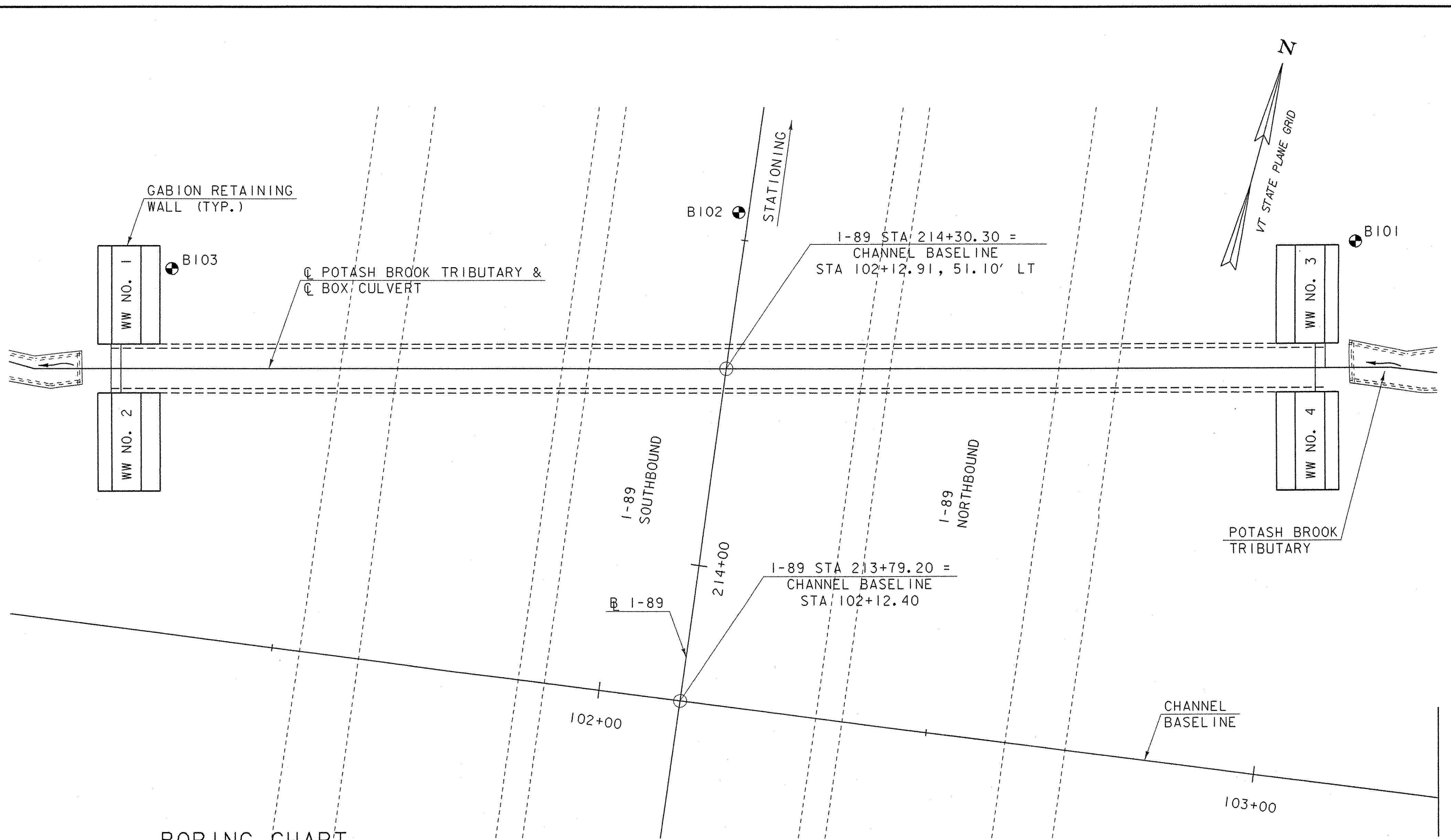
BORING LAYOUT
