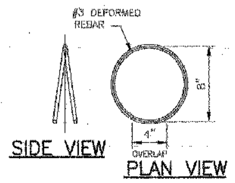
REINFORCING RING DETAIL [A43]
