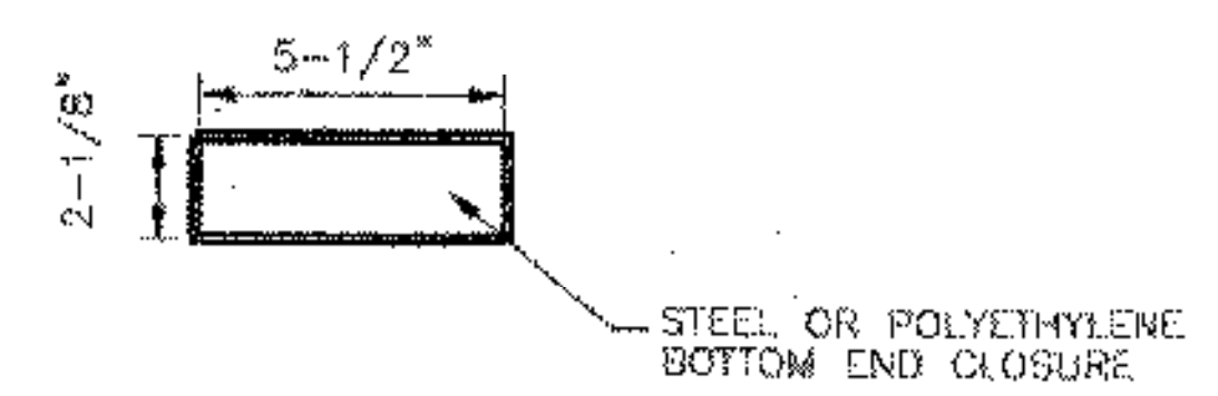
WRGT LARGE SOCKET [W40]
