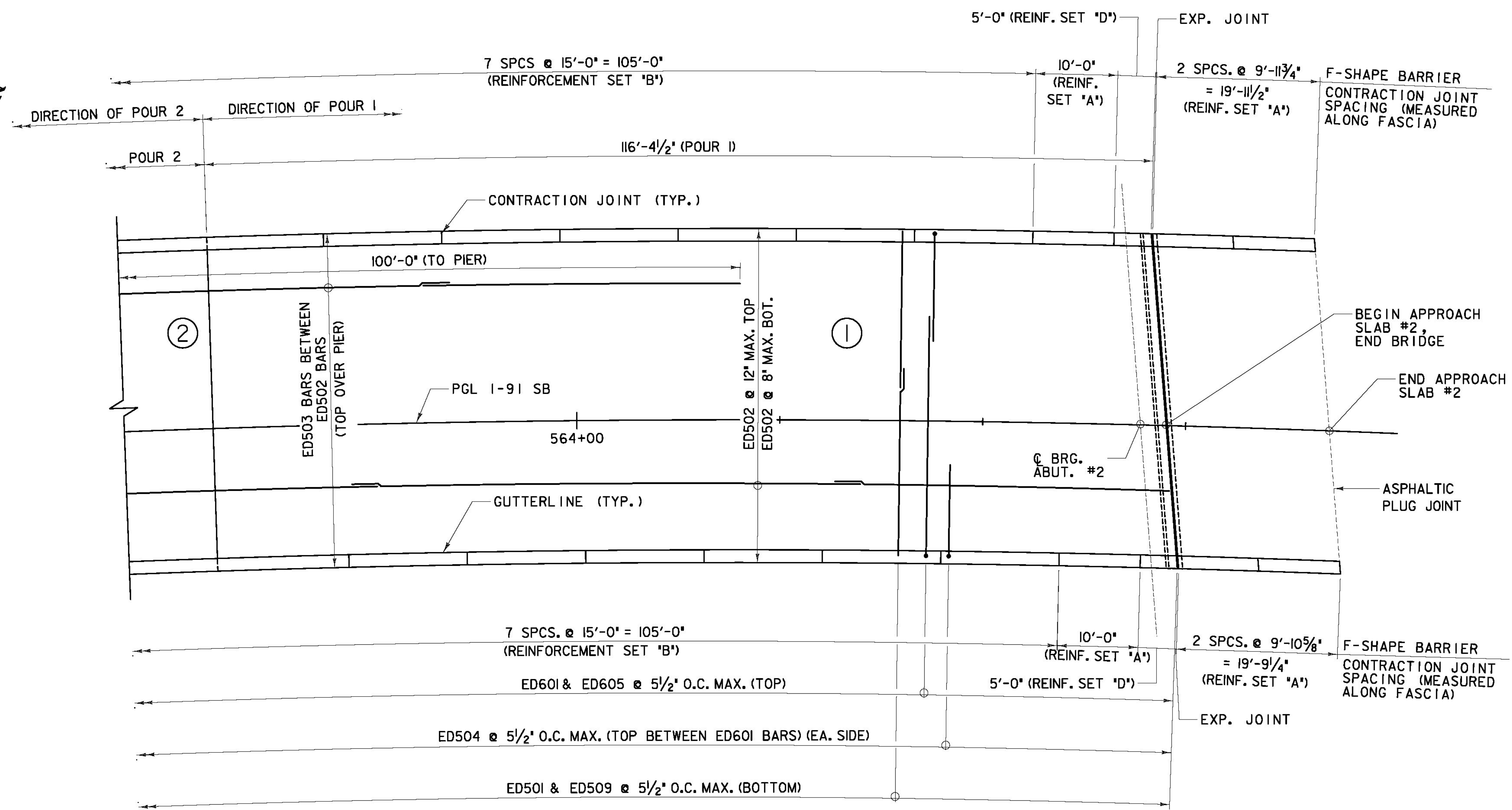
BRIDGE 6S SUPERSTRUCTURE PLAN 3 OF 3 SCALE: 1/8" = 1'-0"
