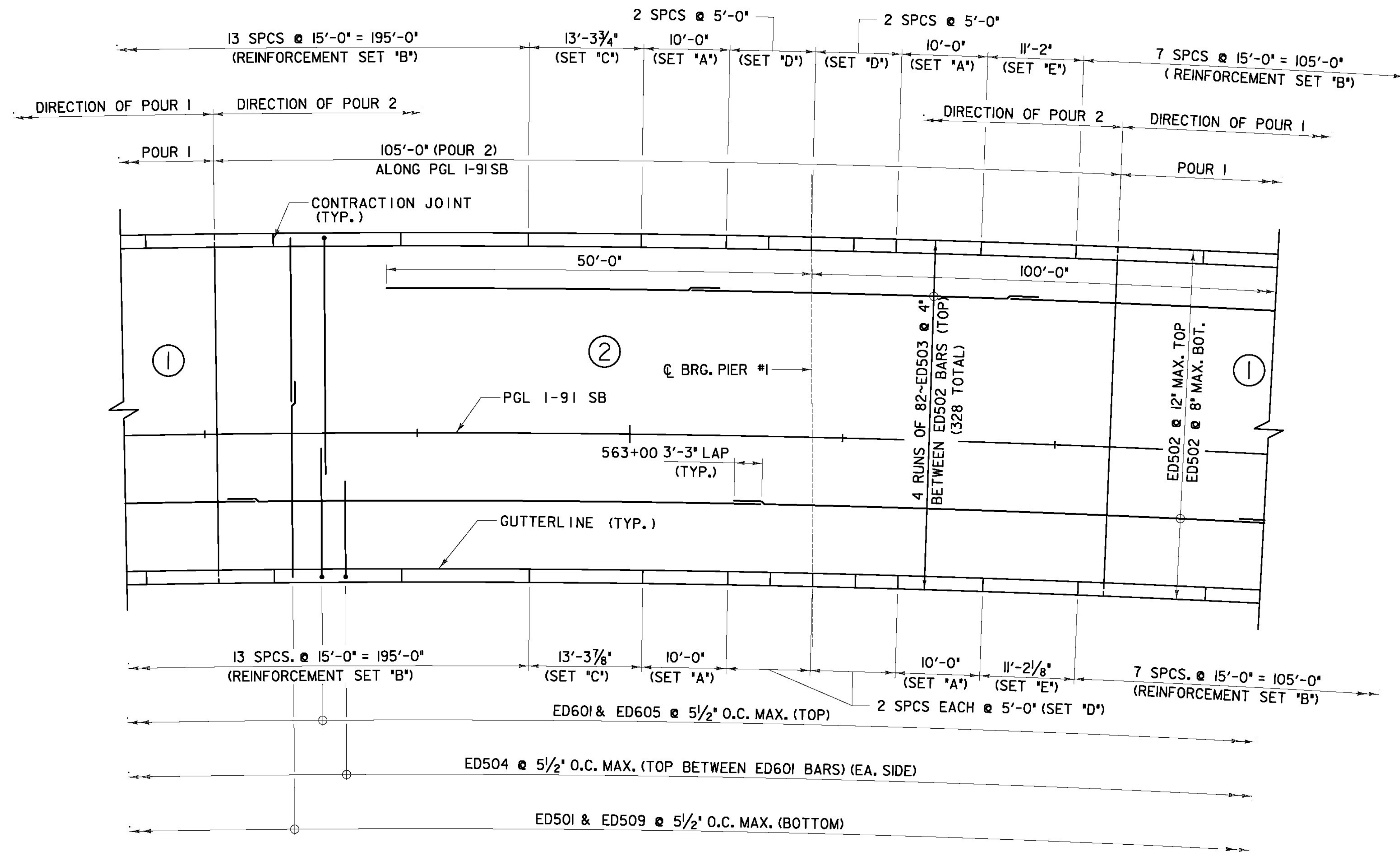
BRIDGE 6S SUPERSTRUCTURE PLAN 2 OF 3 SCALE: 1/8" = 1'-0"
