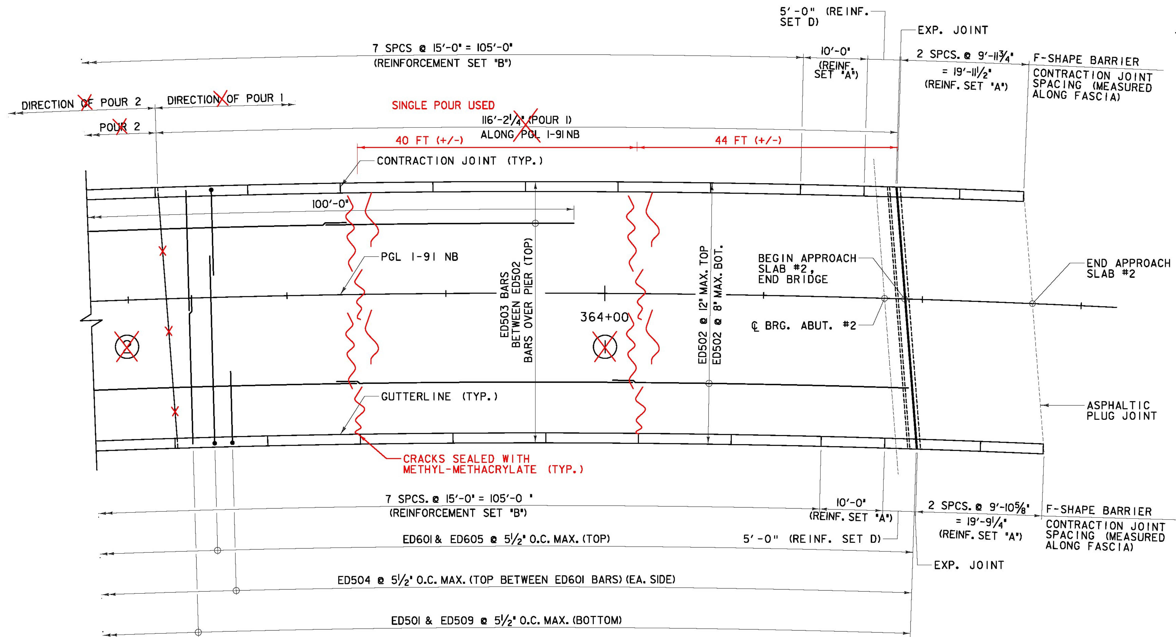
BRIDGE 6N SUPERSTRUCTURE PLAN 3 OF 3 SCALE: 1/8" = 1'-0"
