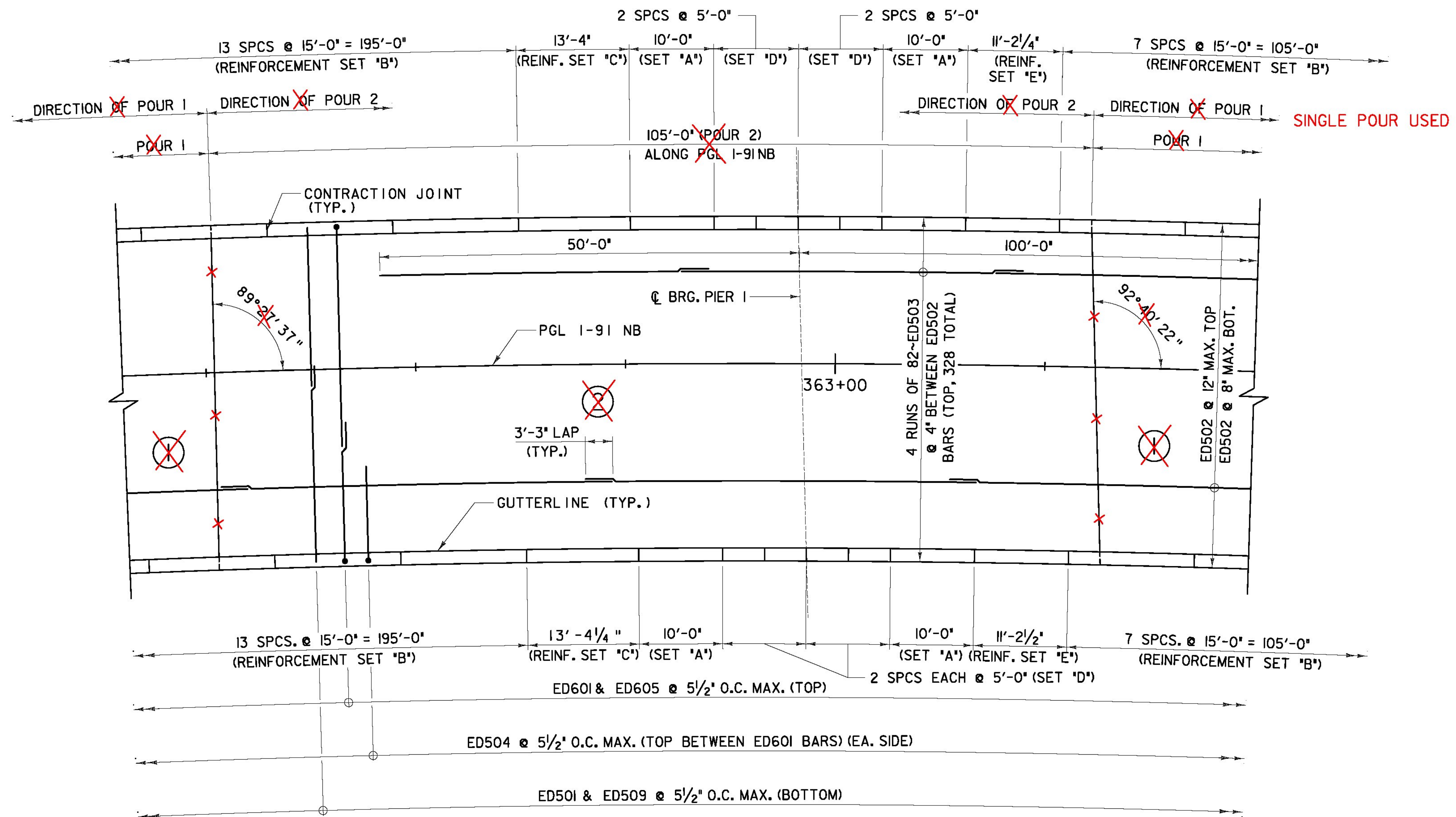
BRIDGE 6N SUPERSTRUCTURE PLAN 2 OF 3 SCALE: 1/8" = 1'-0"
