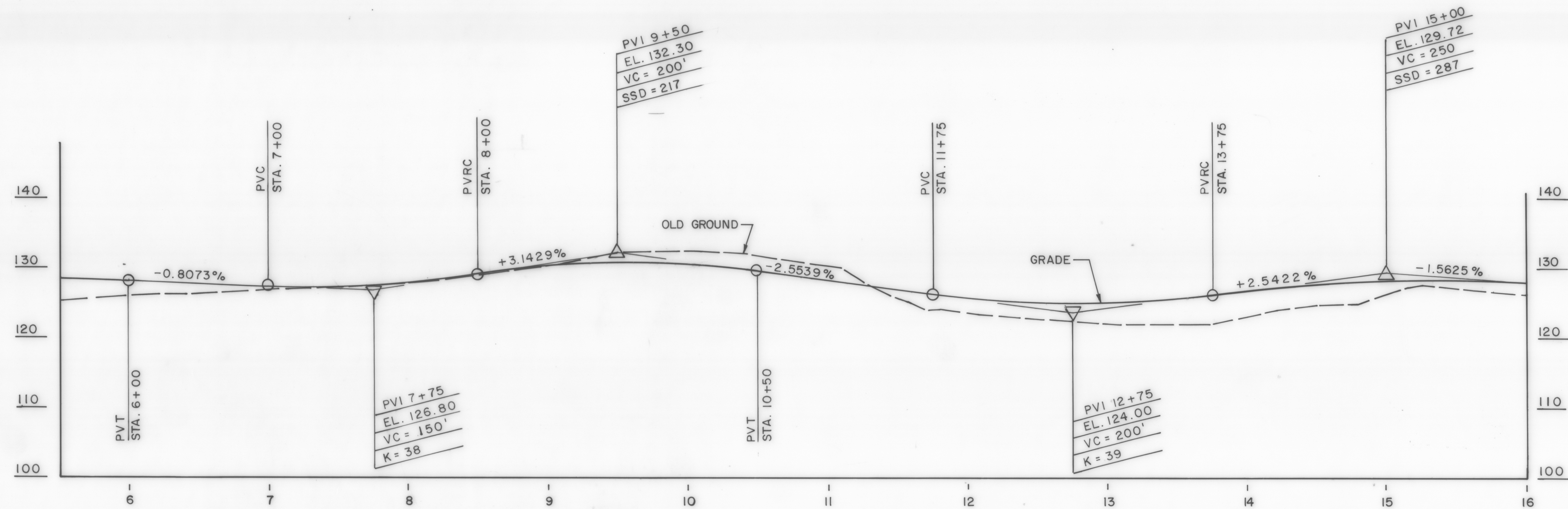
BIKEWAY PROFILE SCALE: 1"=50' H 1"=10' V
