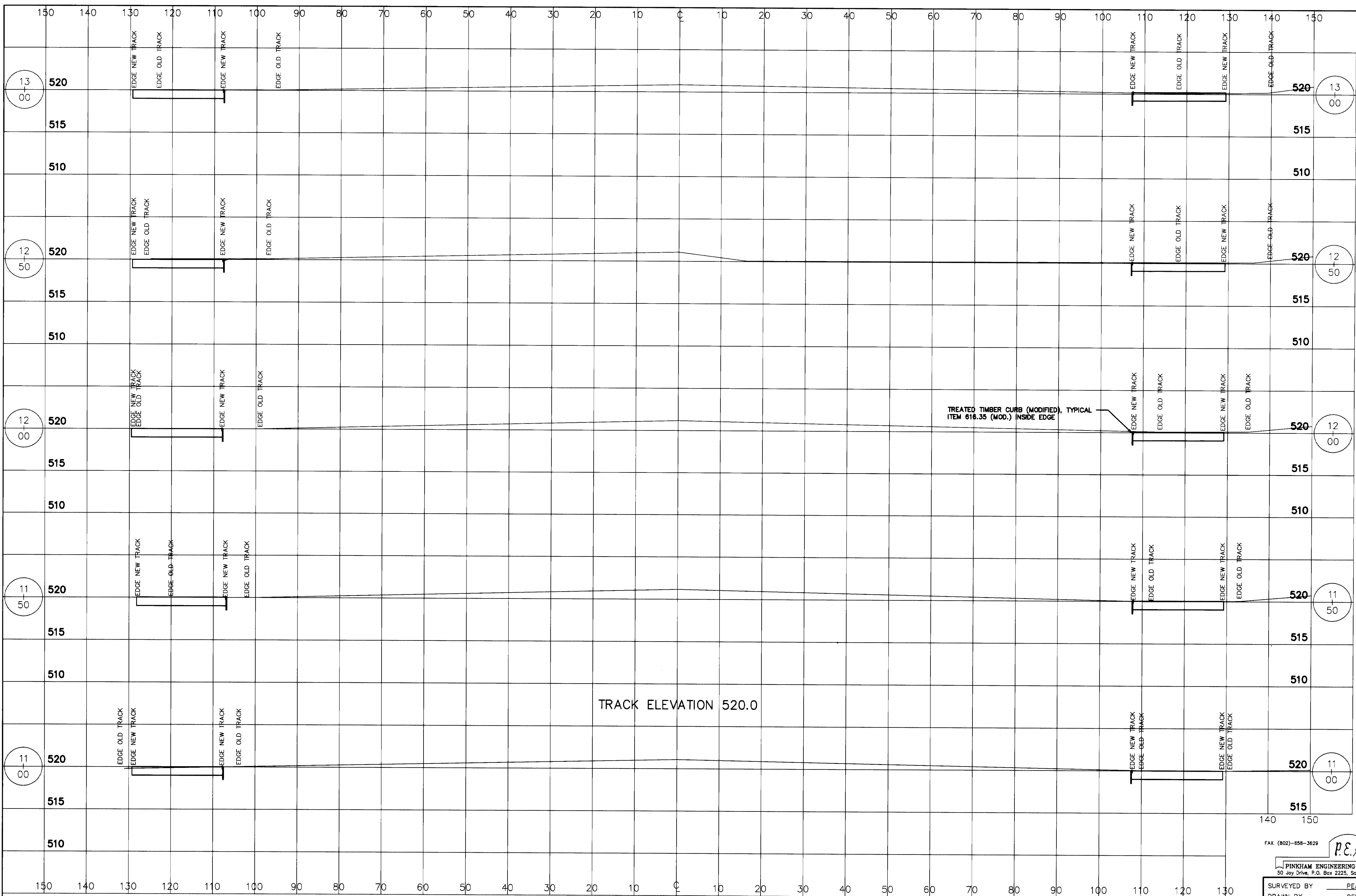
400 METER TRACK SECTIONS SCALE: 1" = 10'
