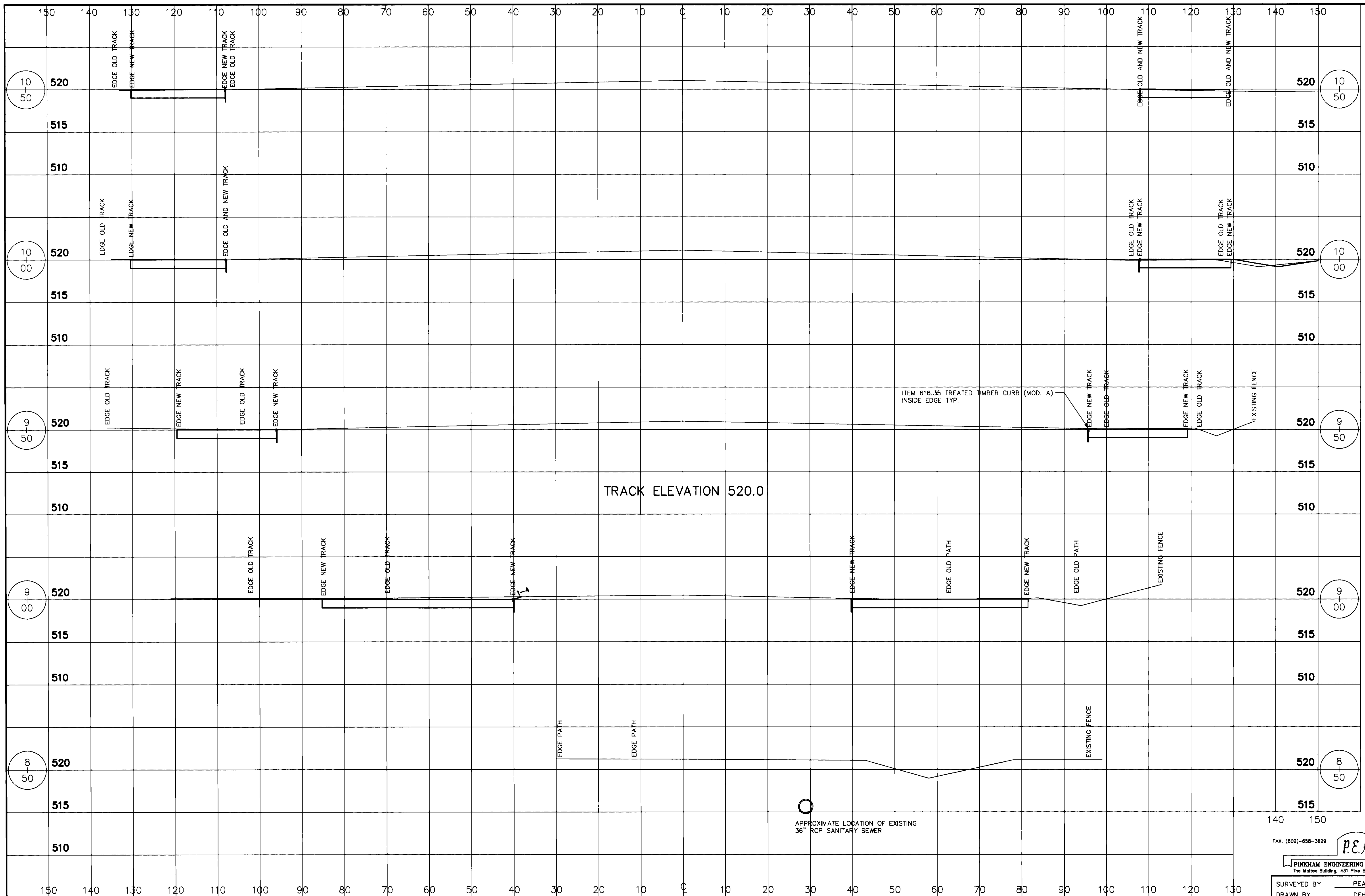
400 METER TRACK SECTIONS 1" = 5' VERT. 1" = 20' HORIZ.
