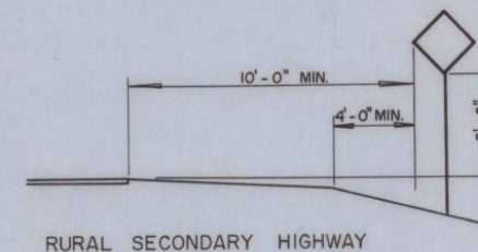
RURAL SECONDARY HIGHWAY
