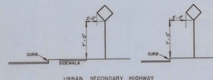
URBAN SECONDARY HIGHWAY
