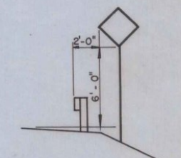
SIGNS ON RAMP
