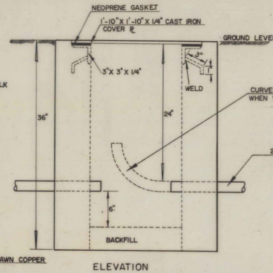
DETAILS OF PULL BOX FOR LIGHTING SYSTEM TYPE "A"
