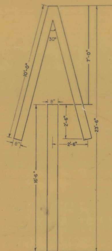
RAMP PAVEMENT ARROW DETAIL
