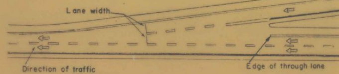
TAPERED ACCELERATION LANE
