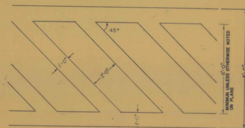
CROSSWALK DETAIL
