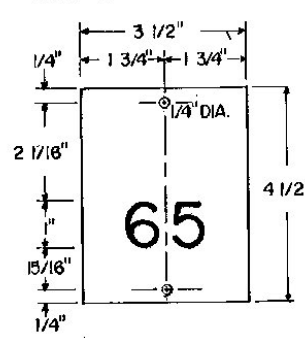
MILEPOST PLAQUE PART "A" (THE NUMERALS ON PART "A" INDICATE THE MILE.)
