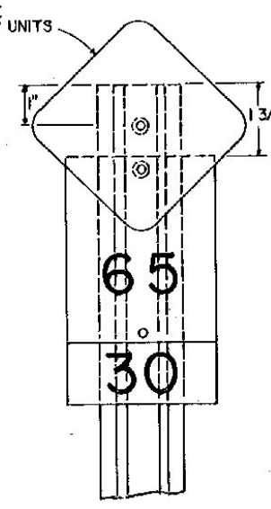
TYPE I WITH PLAQUE
