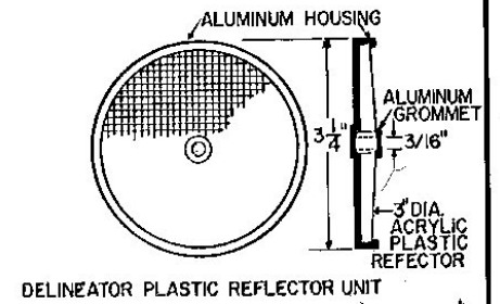
DELINEATOR PLASTIC REFLECTOR UNIT
