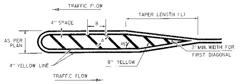
PAINTED ISLAND DETAIL
