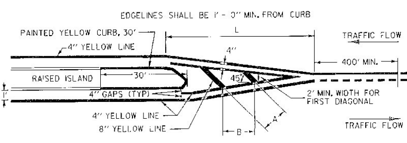
ISLAND APPROACH MARKINGS
