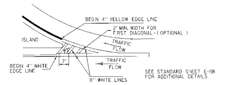
GORE MARKING DETAIL - EXIT TRANSVERSE LINES
