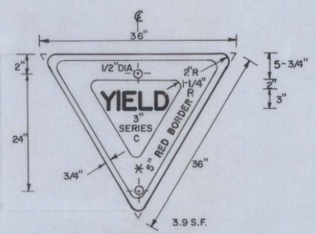
RED REFLECTORIZED BORDER ON A REFLECTORIZED WHITE BACKGROUND WITH RED PAINTED TEXT, REVERSE SCREENED METHOD.
