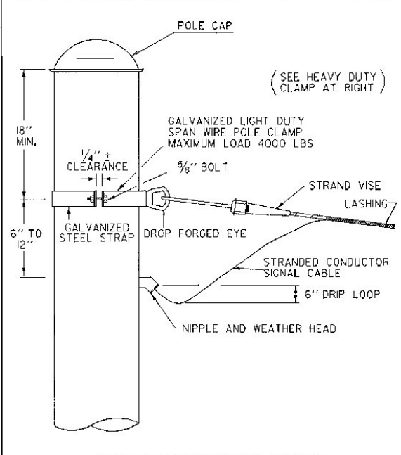
CABLE INSTALLATION TYPICAL WITH SPAN WIRE POLE CLAMP (LIGHT DUTY GALVANIZED)
