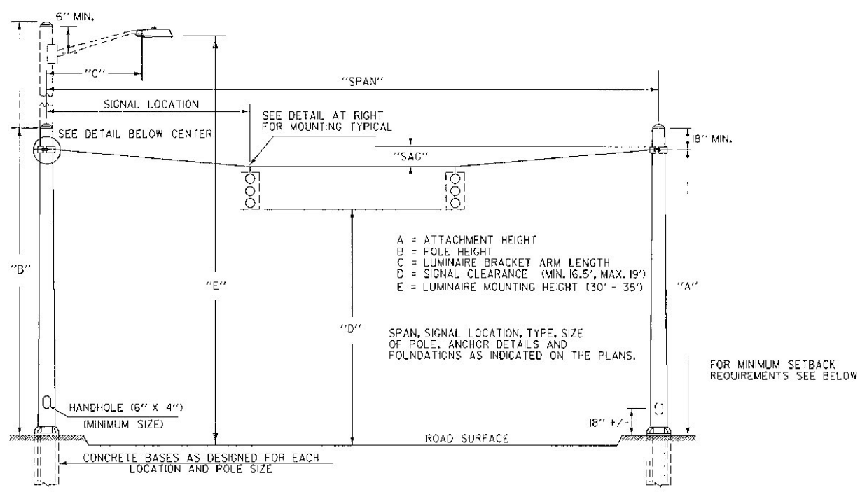
SPAN WIRE MOUNTED TRAFFIC SIGNALS WITH LUMINAIRES
