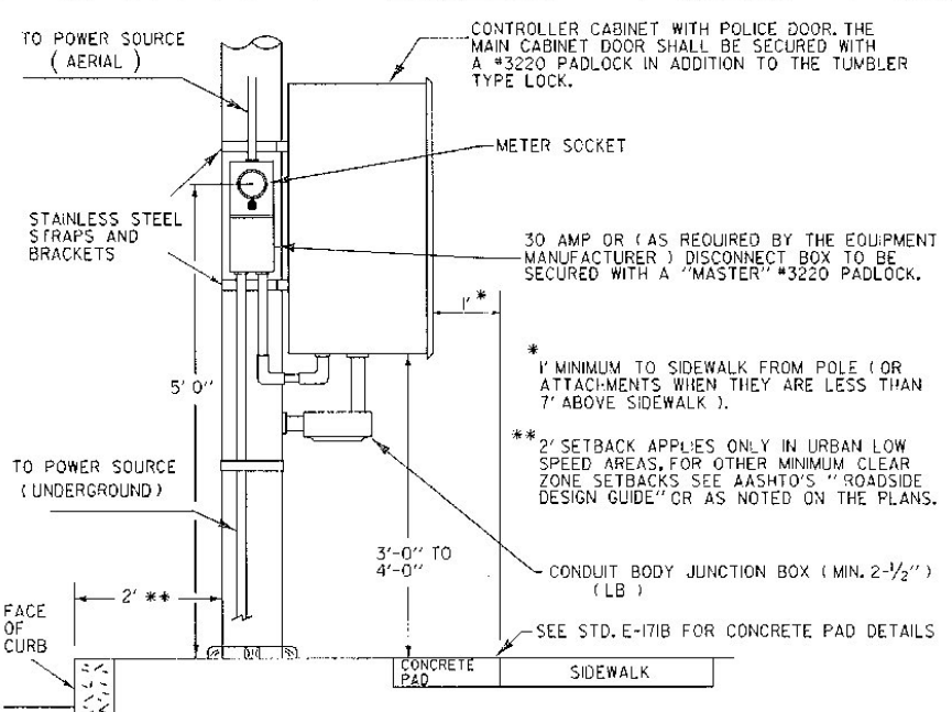
POLE MOUNTED CONTROLLER CABINET INSTALLATION TYPICAL
