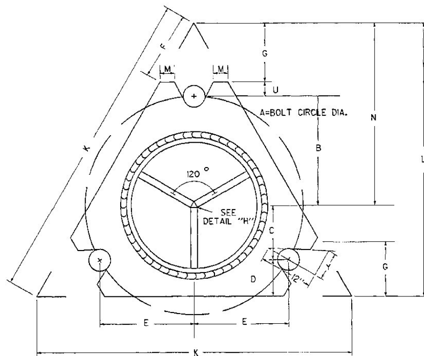
DETAILS OF MULTI-DIRECTIONAL SLIP BASE
