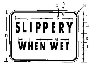
* REDUCE LETTER SPACING 25% W8-10A
