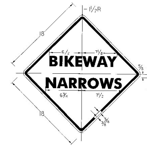
* REDUCE LETTER SPACING 50% W5-4A
