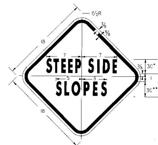
* REDUCE LETTER SPACING 60% ** REDUCE LETTER SPACING 75% VW-560
