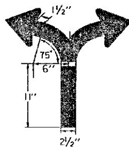
SYMBOL DETAILS
