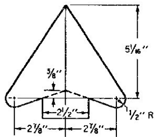
ARROW HEAD DETAIL
