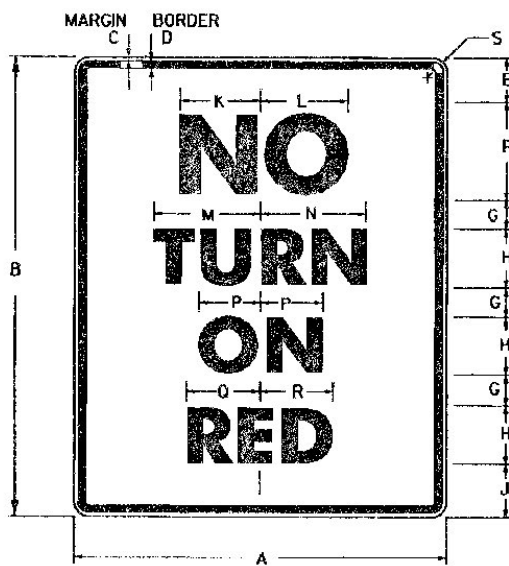
POST MOUNTING R10-11A
