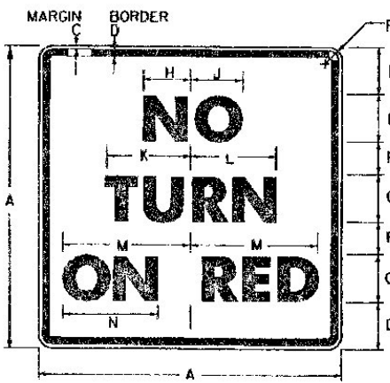
OVERHEAD MOUNTING R10-11B
