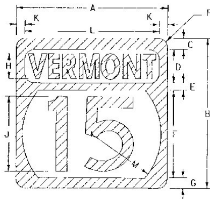
1 OR 2 DIGIT STATE ROUTE MARKER
