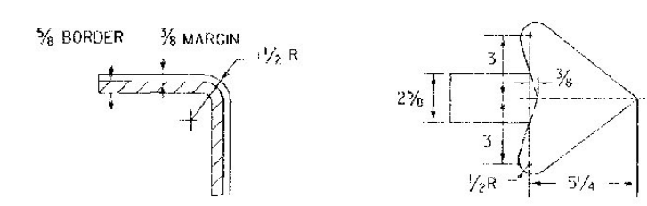
TYPICAL RADIUS DETAIL TYPICAL ARROW DETAIL
