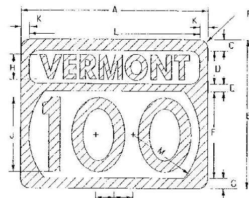
3 DIGIT STATE ROUTE MARKER
