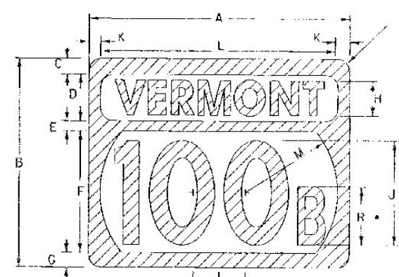
3 DIGIT ALTERNATE STATE ROUTE MARKER
