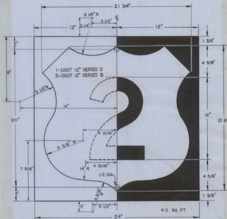
U. S. ROUTE MARKER FOR INDEPENDENT USE WITH MARKER ASSEMBLIES
