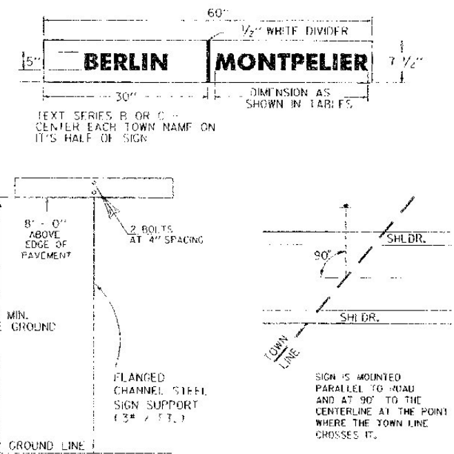
TOWN LINE POST TOWN LINE SIGN WHEN CROSSING COUNTY BOUNDARIES AN ADDITIONAL COUNTY LINE SIGN SHALL BE MOUNTED BELOW THE TOWN LINE SIGN.
