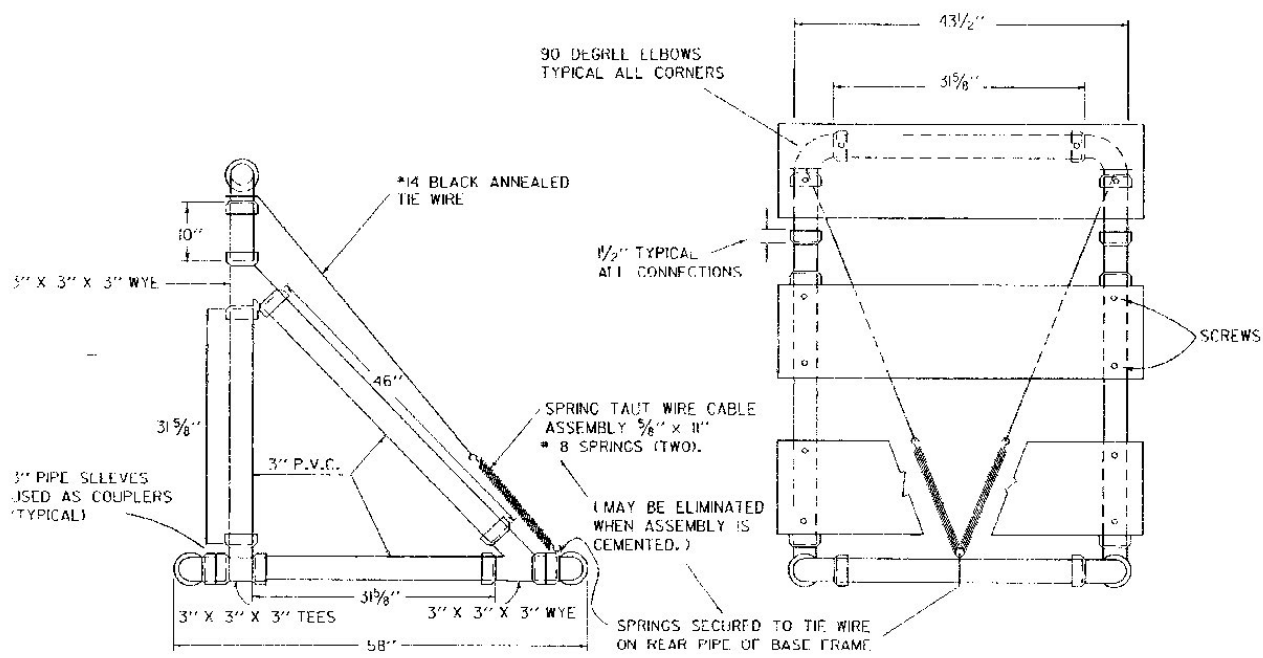
SIDE VIEW TYPE III BARRICADE
