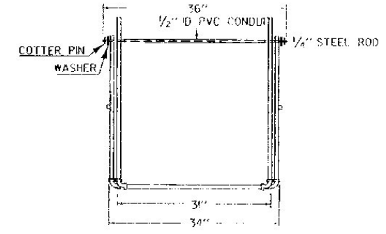
TYPE I AND TYPE II BARRICADE
