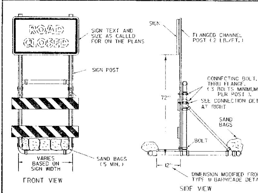
SIGN MOUNTING ON TYPE III BARRICADE (MODIFIED)
