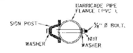
CONNECTION DETAIL
