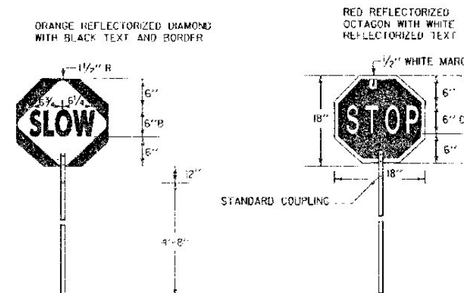
SIGN DETAIL
